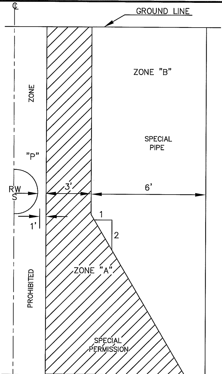
CASE 2 NEW POTABLE WATER OR NEW RECYCLED WATER
